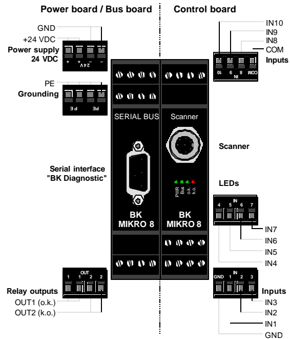
Fig. 2-1: Control unit – front view with connections
