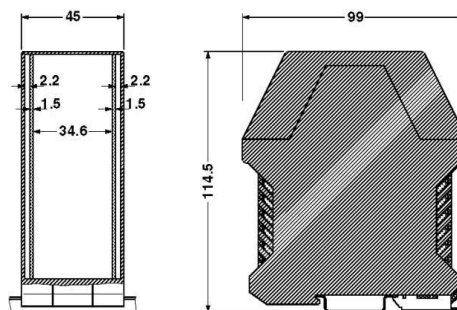
General tolerances ISO 2768 – mK
