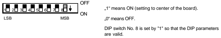
Fig. 2-6: DIP switch S1
